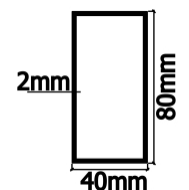
Roof tension tube
