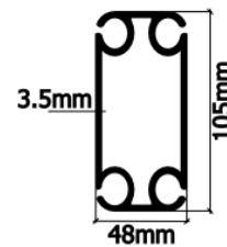
Main frame profile
