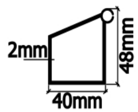
Eave purlin
